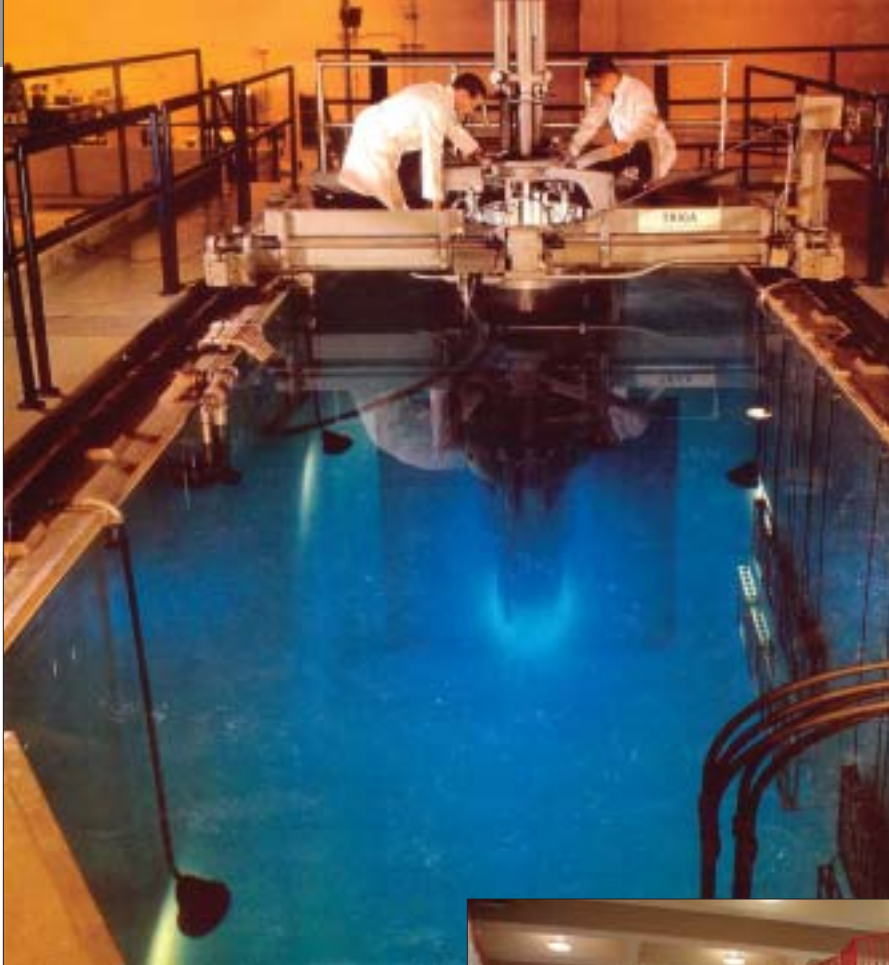
Fig. 14. TRIGA movable core reactor at Northrop Corp., in California
