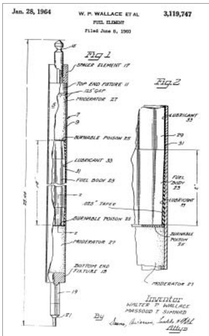
Fig. 5. U.S. Patent No. 3,119,747, filed June 8, 1960
