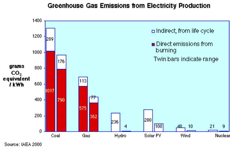
Fig.2: Results of life-cycle analyses for CO 2 emission from electricity generation by various methods (Source: [5])
