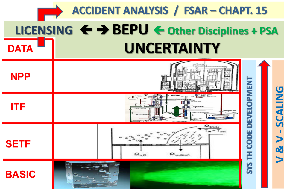
Fig. 1 – The BEPU process focusing on Accident Analysis and Chapter 15 of FSAR (NOTE: Acronyms and symbols in the figure not defined in the paper are, in alphabetic order: ITF = Integral Test Facility; SETF = Separate Effect Test Facility; SYS TH = System Thermal-Hydraulics; V & V = Verification and Validation; \dot{M}_{ECC} = Mass flow-rate of injected Emergency Core Cooling; \dot{M}_{w,COND} = Condensed mass flow-rate penetrating the core; \dot{M}_{s,G} = Upward mass flow-rate of steam and gas; T_{sat} = saturation temperature; T_w = water temperature).
