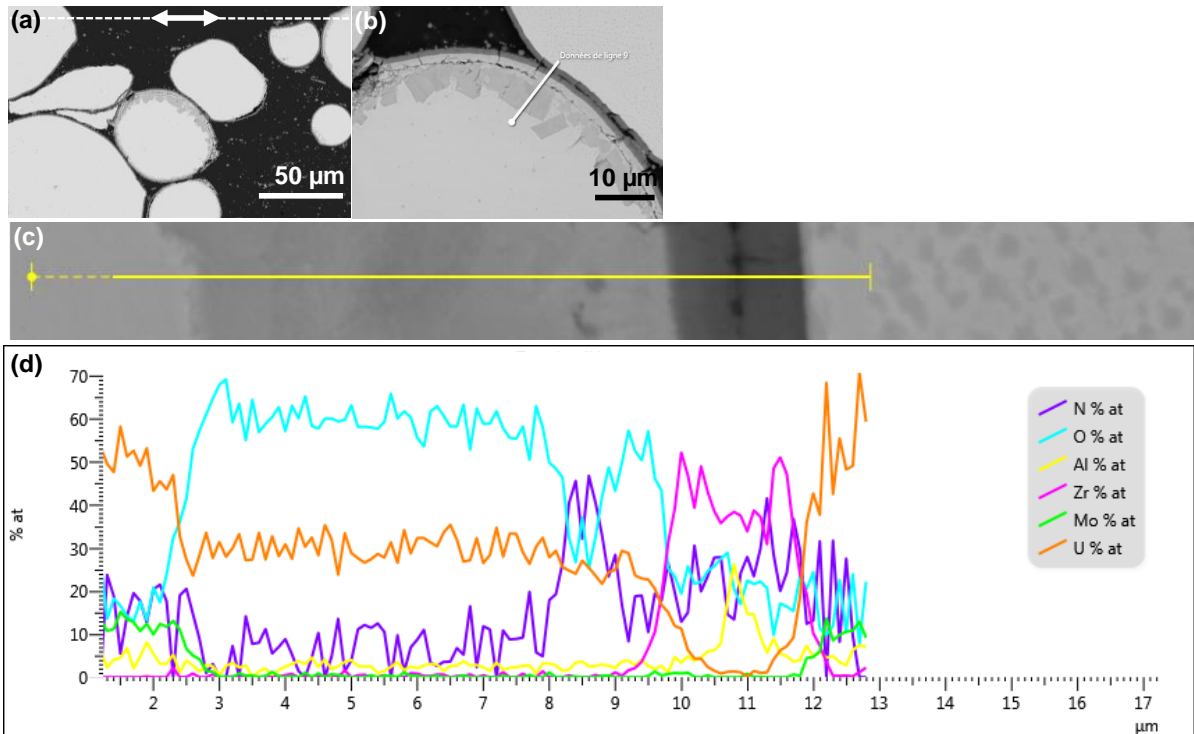
Figure 6: SEM/EDS analysis of an oxidized U(Mo) particle in SF-202 plate (a) general view (white arrow: rolling direction – dashed line: approximate position of fuel-cladding interface), (b) and (c) location of the analysis line, (d) EDS profiles along the yellow line drawn in (c).
